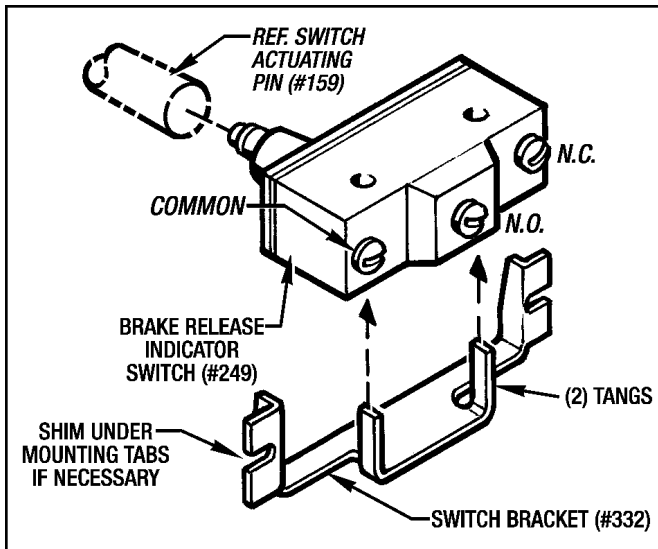
Figure 7.16 - Brake Release Indicator Switch
