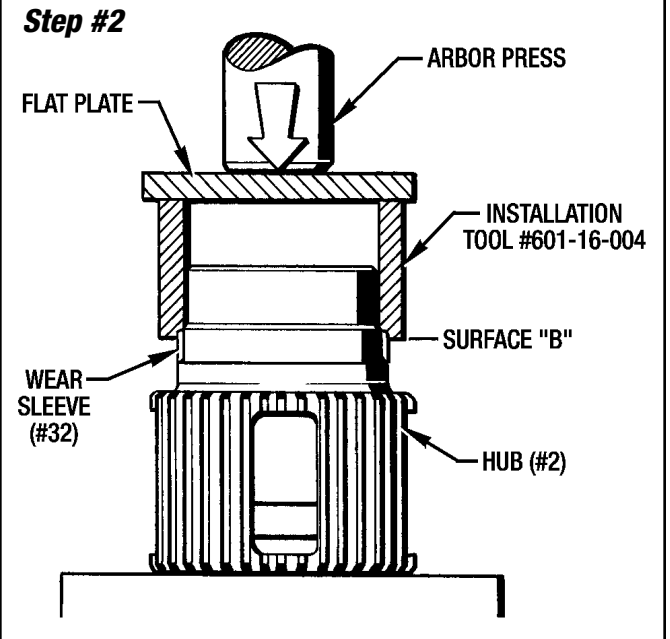
Figure 7.12 - Installing Wear Sleeve (#32) on Sizes MSB9 and MSB10
