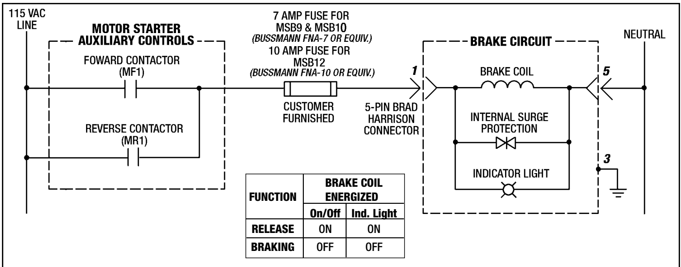
Figure 3.8 - Electrical Schematic
