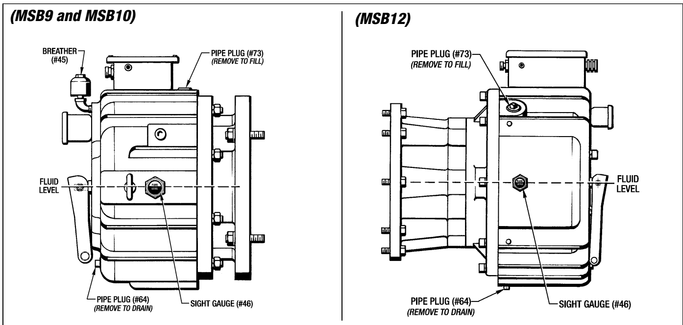
Figure 4.1 - Lubrication - Horizontal Mounting
