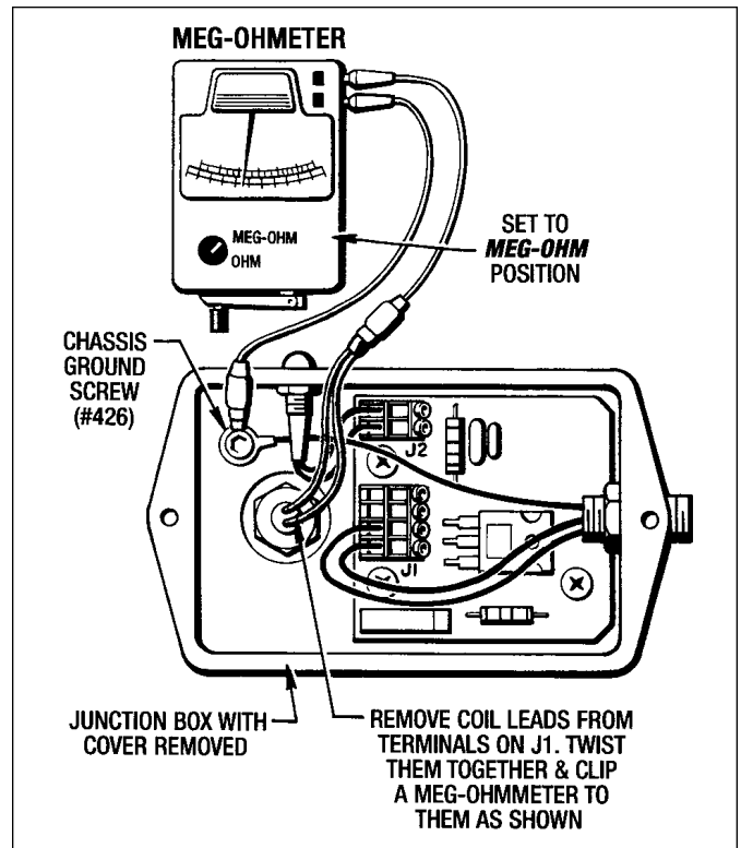
Figure 6.2 - Coil Current Leakage Testing
