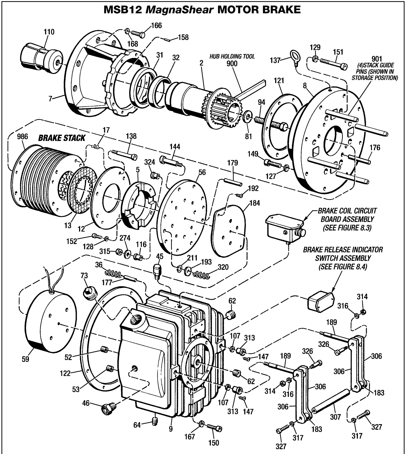
Figure 8.2 Repair Parts - MSB12 MagnaShear Motor Brake
