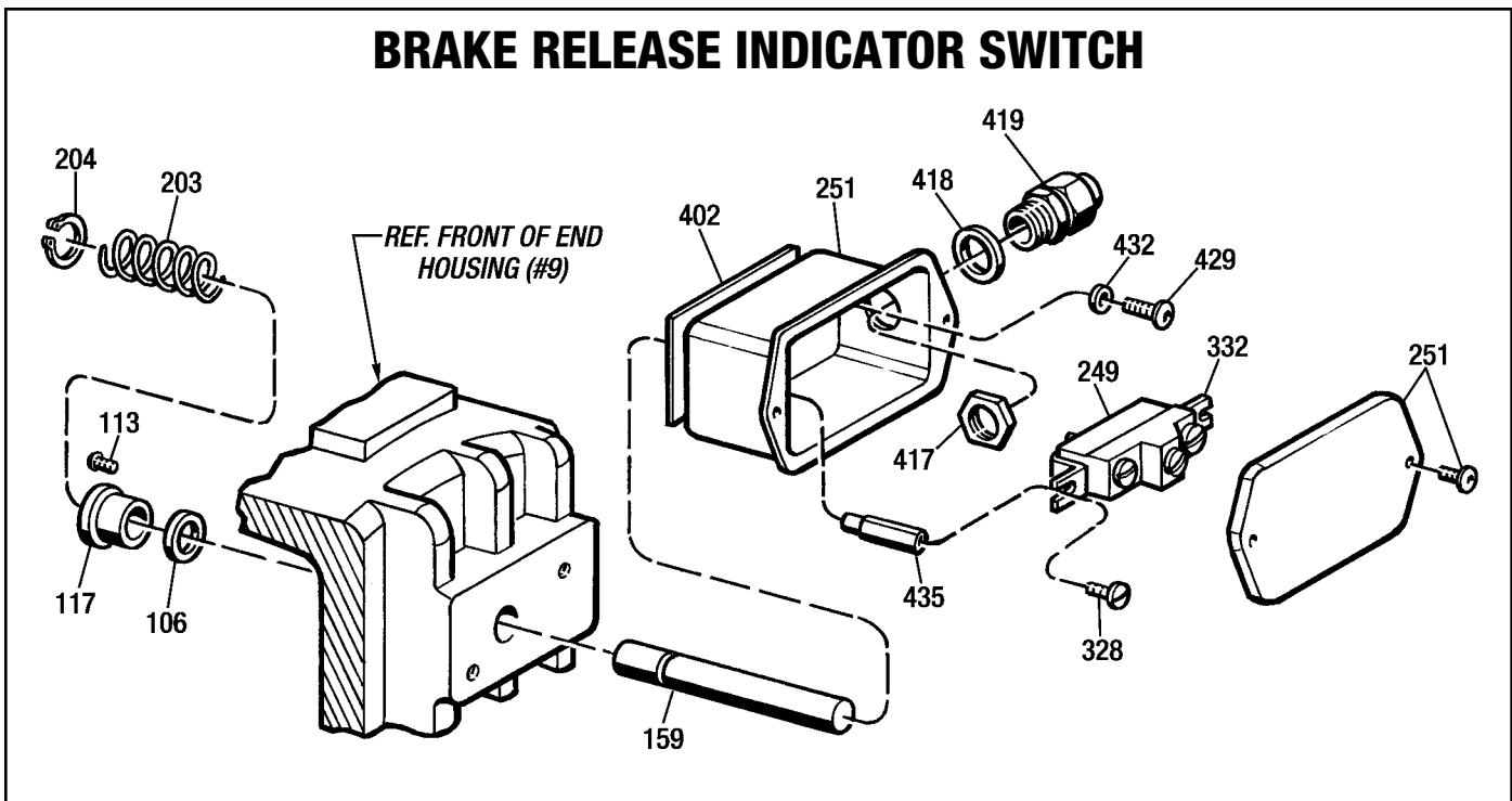
Figure 8.4 - Brake Release Indicator Switch
