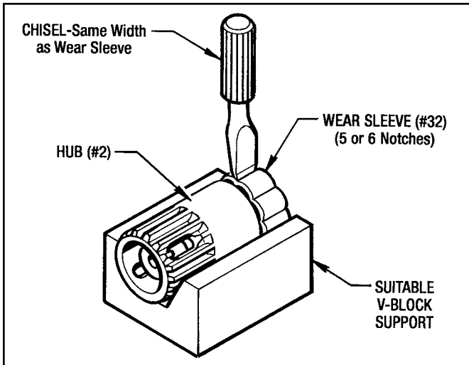
Figure 7.10 - Removing Wear Sleeve (#32)
