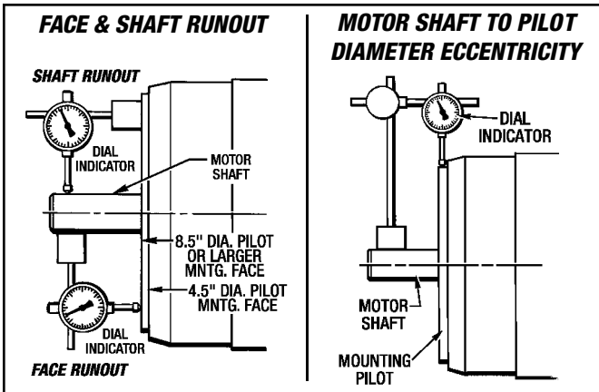
Figure 3.3 - Verifying Motor Specifications
