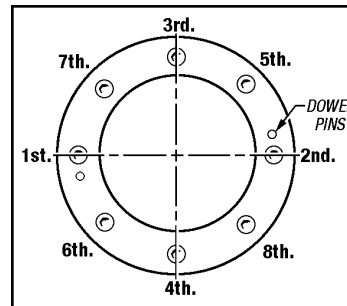
Figure 3.2 - Torque Pattern Example
