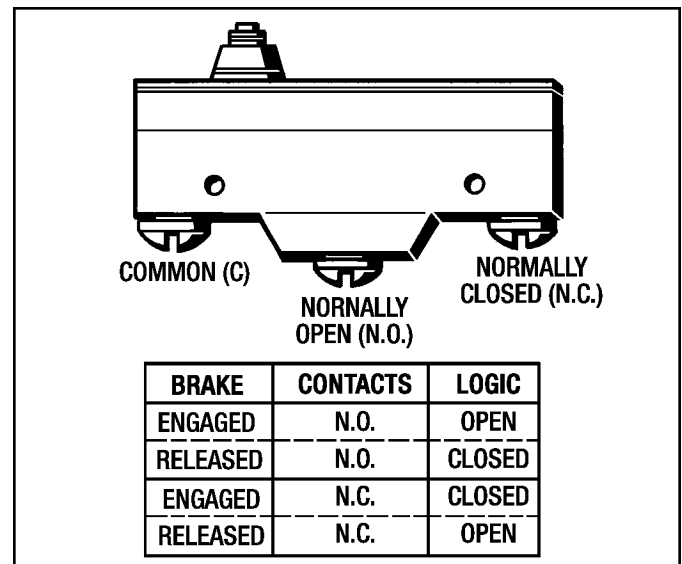
Figure 3.10 - Brake Release Indicator Switch
