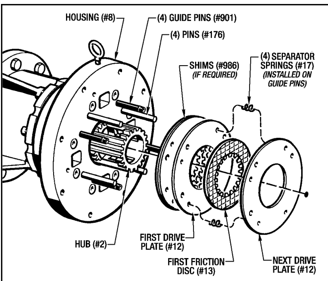
Figure 3.7 - Installing MSB12 Brake Stack
