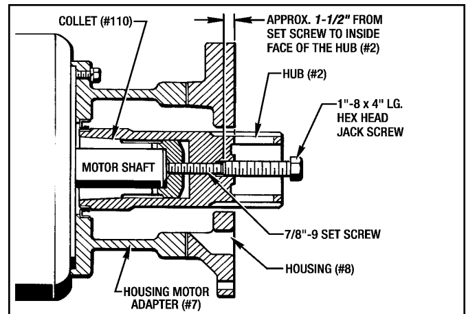
Figure 7.9 - Removing Hub (#2) for MSB12
