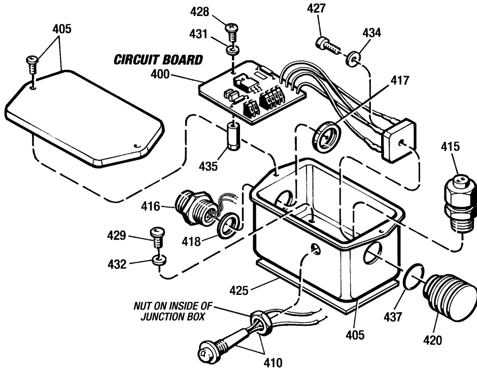
Figure 8.3 - Electric Box and Circuit Board
