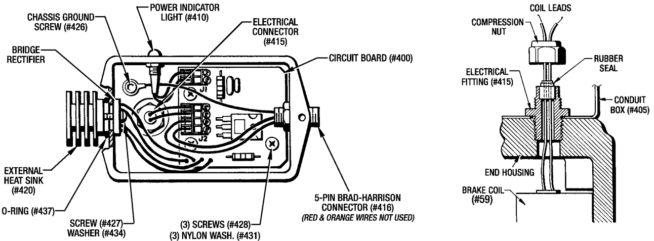
Figure 7.6 - Conduit Box with Cover Removed for Size MSB12 Motor Brake
