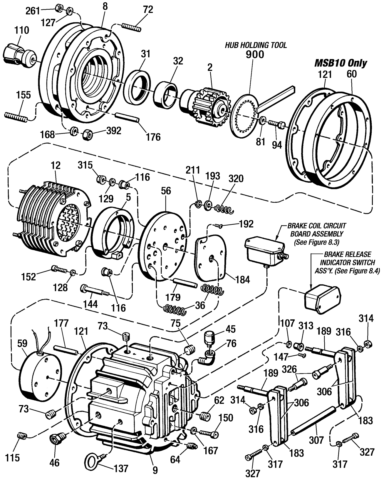
Figure 8.1 - Repair Parts - MSB9 and MSB10 MagnaShear Motor Brake
