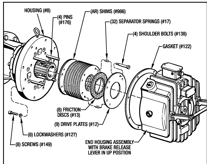
Figure 7.3 - Removing MSB12 Brake Stack
