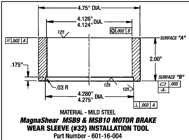
Figure 7.11 - Wear Sleeve Installation Tool
