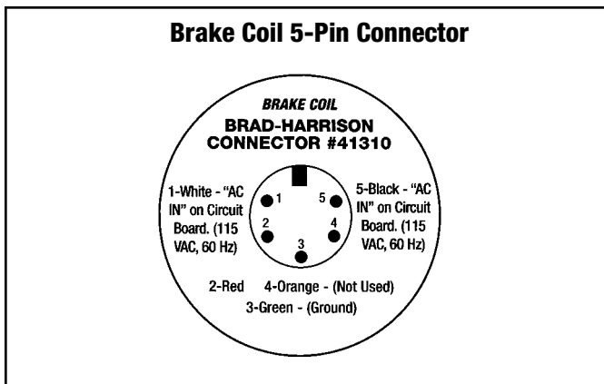
Figure 3.9 - Brad Harrison Connectors
