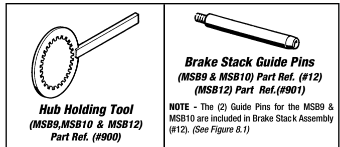
Figure 3.1 - Special Assembly Tools
