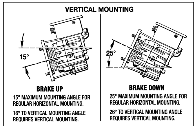
Figure 3.6 - Vertical Mounting
