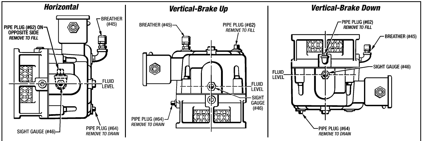
Figure 4.2 - Lubrication - MSB4 MagnaShear
