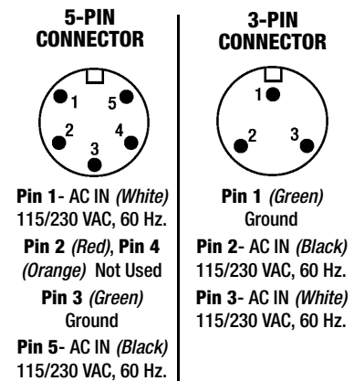
Figure 3.8 - Electrical Connector
