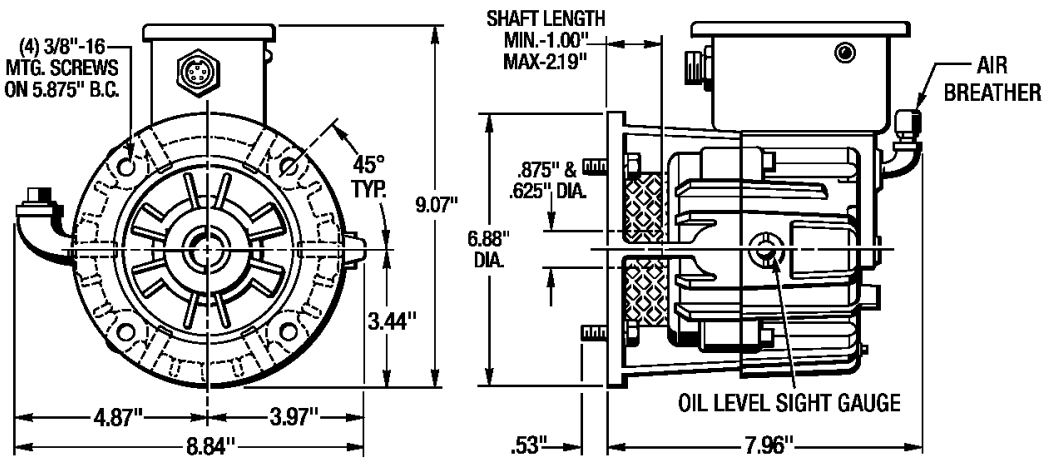
Figure 2.1 - Dimensions
