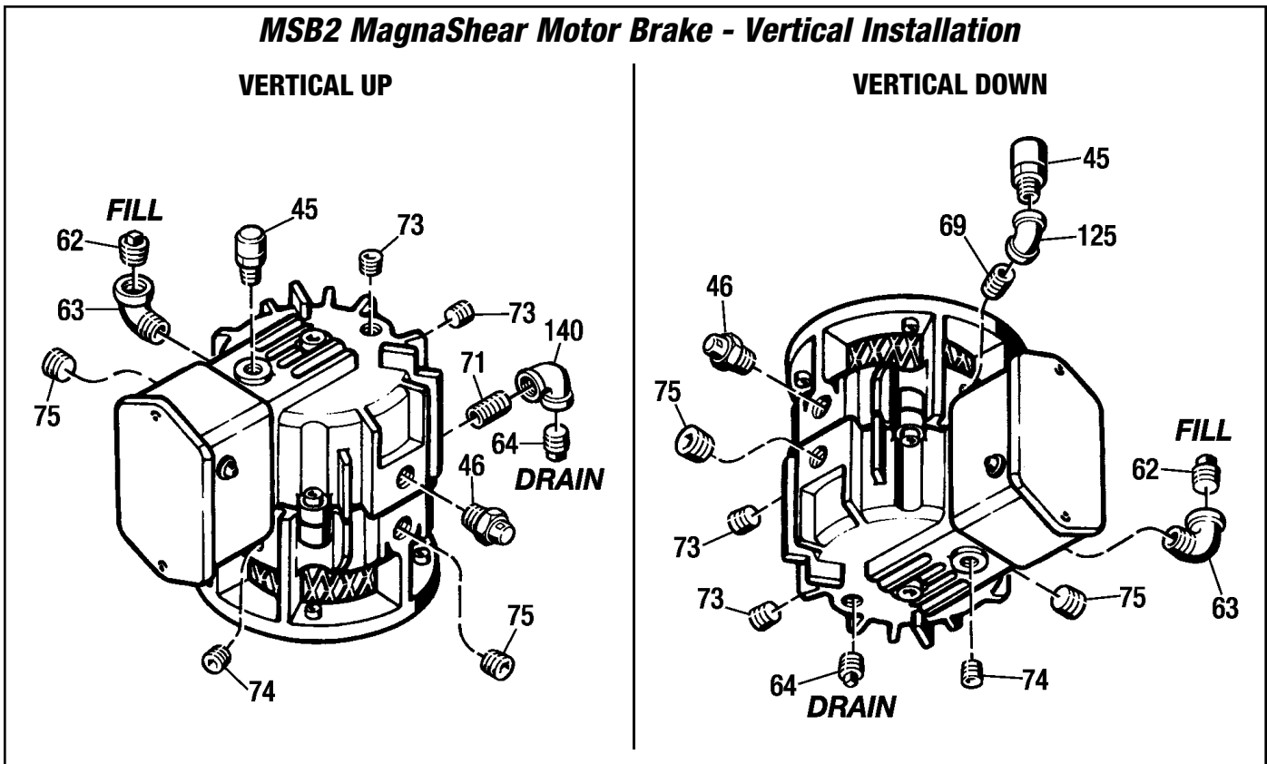
Figure 8.5 - MSB2 MagnaShear Motor Brake - Vertical Installation
