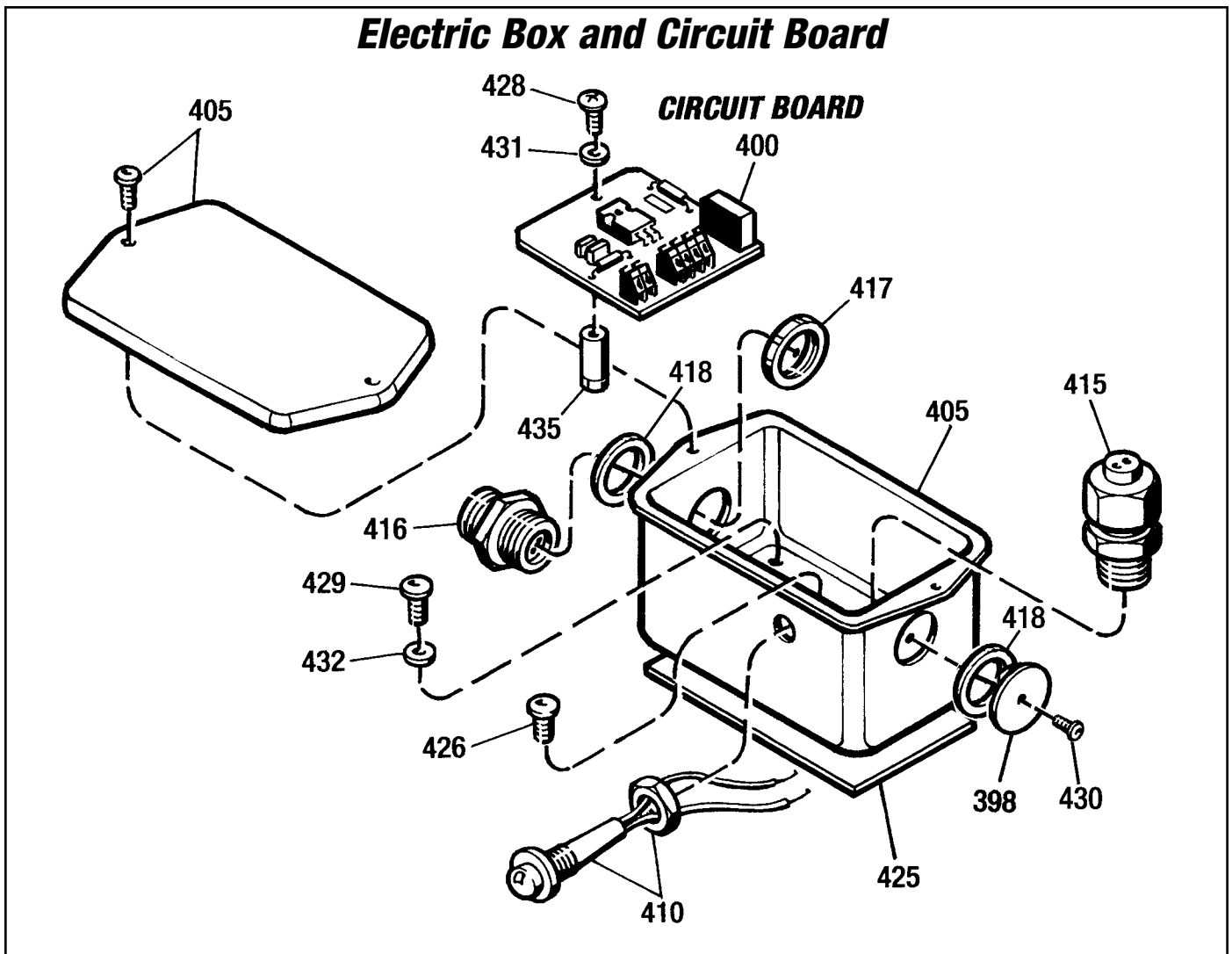
Figure 8.1 - Electric Box and Circuit Board
