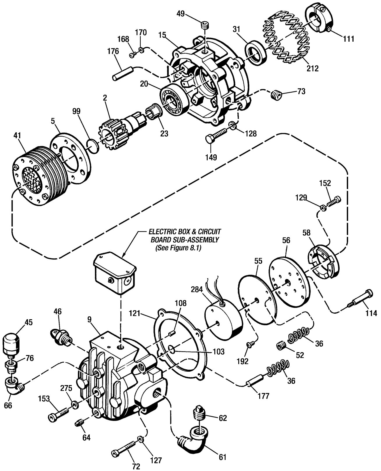
Figure 8.3 - MSB4 "Quick Mount" MagnaShear Motor Brake
