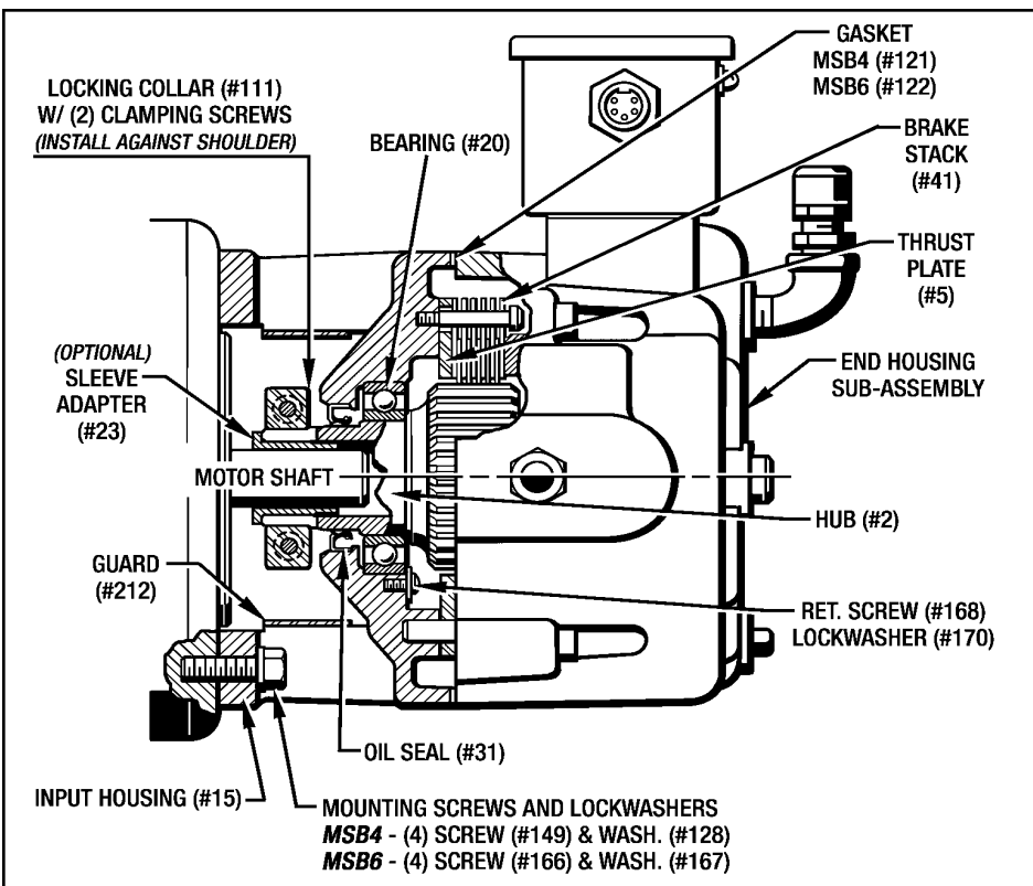
Figure 7.9 - Installing MSB4 and MSB6 Back On Motor
