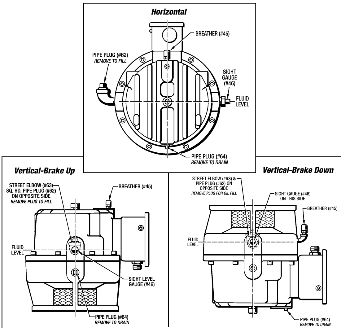
Figure 4.3 - Lubrication - MSB6 MagnaShear
