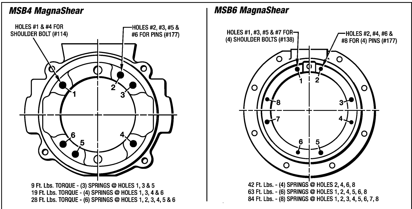
Figure 7.7 - Spring Placement for MSB4 and MSB6
