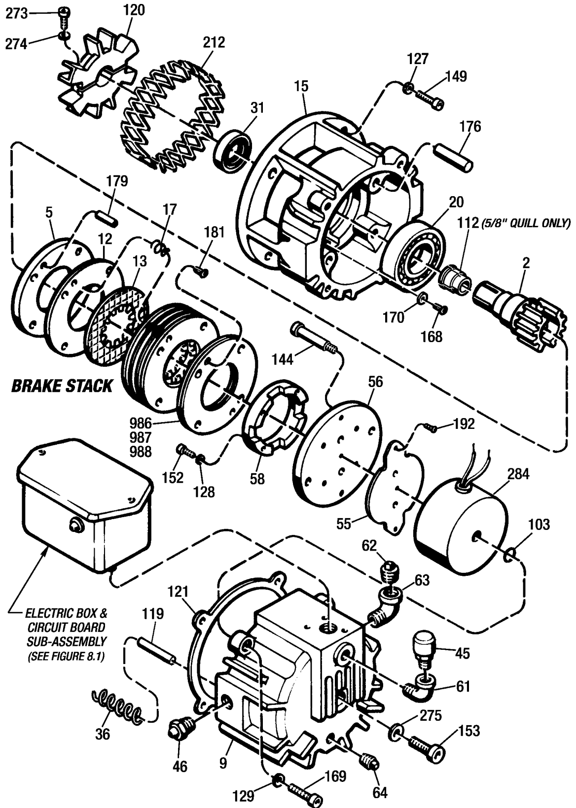
Figure 8.2 - Repair Parts - MSB2 MagnaShear Motor Brake
