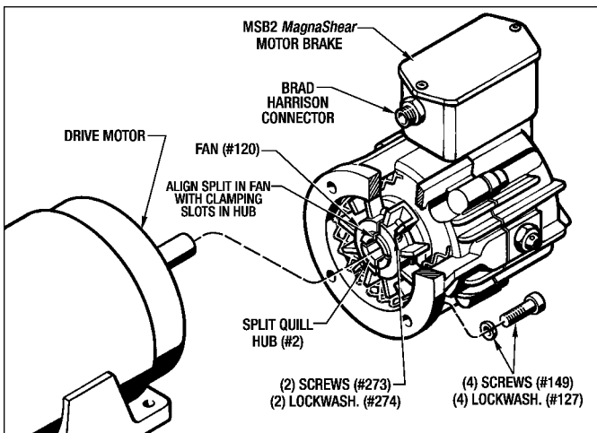
Figure 3.3 - Installing The MSB2 Onto The Drive Motor
