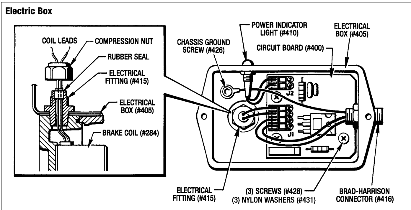
Figure 7.5 - Electric Box with Cover Removed
