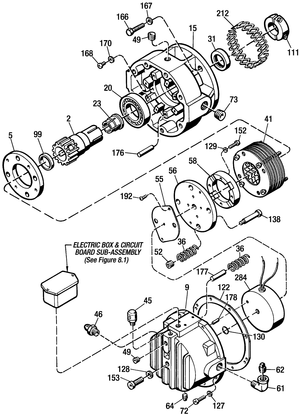
Figure 8.4 - MSB6 "Quick Mount" MagnaShear Motor Brake
