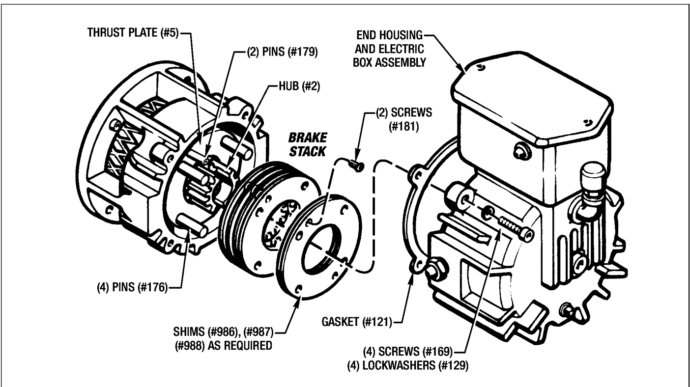
Figure 7.3 - Replacing the Brake Stack - MSB2 MagnaShear
