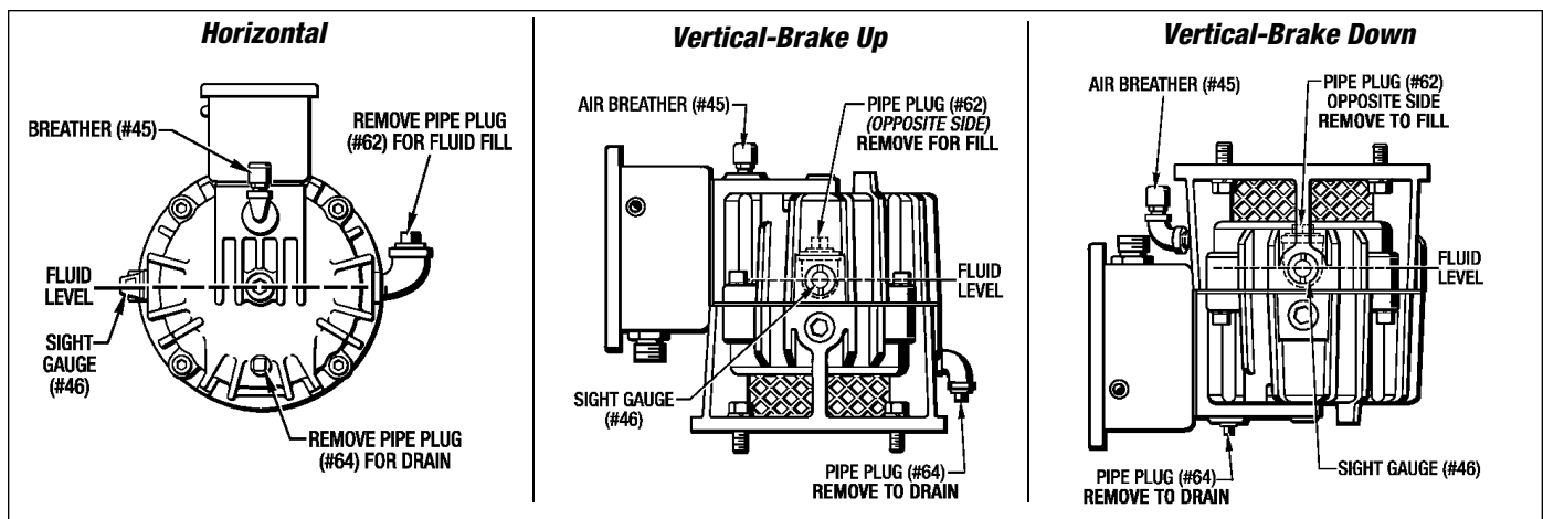
Figure 4.1 - Lubrication - MSB2
