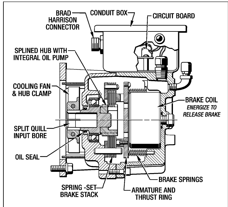
Figure 1.2 - MagnaShear "Quick Mount" Motor Brake Cross Section
